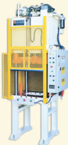
STP-30 TONS
