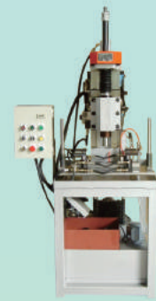
HD-320油壓滑座自動鑽孔機 S45C-φ32 Hydraulic Slide-Base Automatic Drilling Machine S45C-φ32
