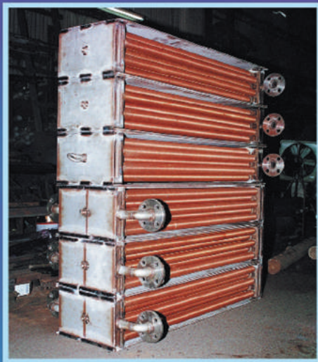
▲ Steam/Air Heat Exchangers (brass and stainless-steel) 蒸氣/空氣熱交換器(銅X白鐵)
